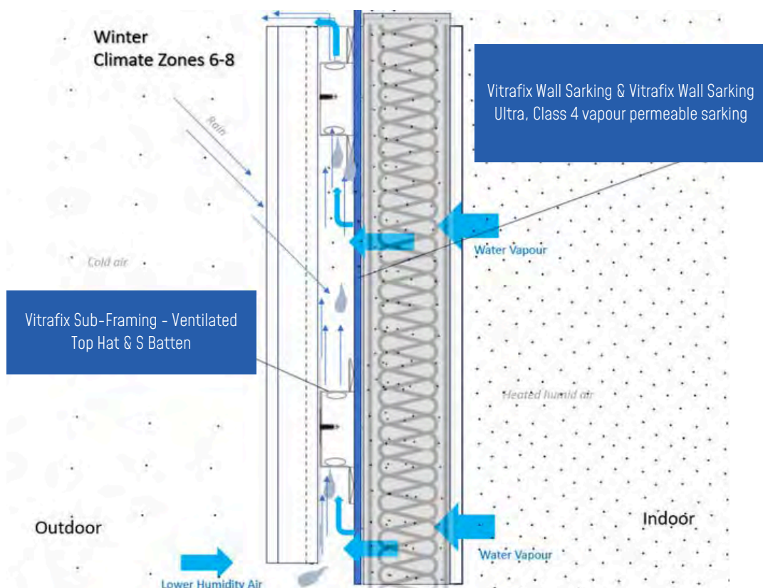
Water vapour escaping into the rainscreen cavity
