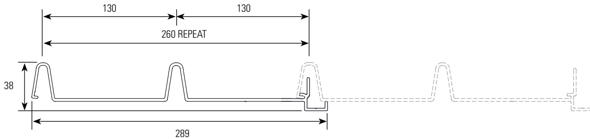
SEAM 130/130 - SE130/130
